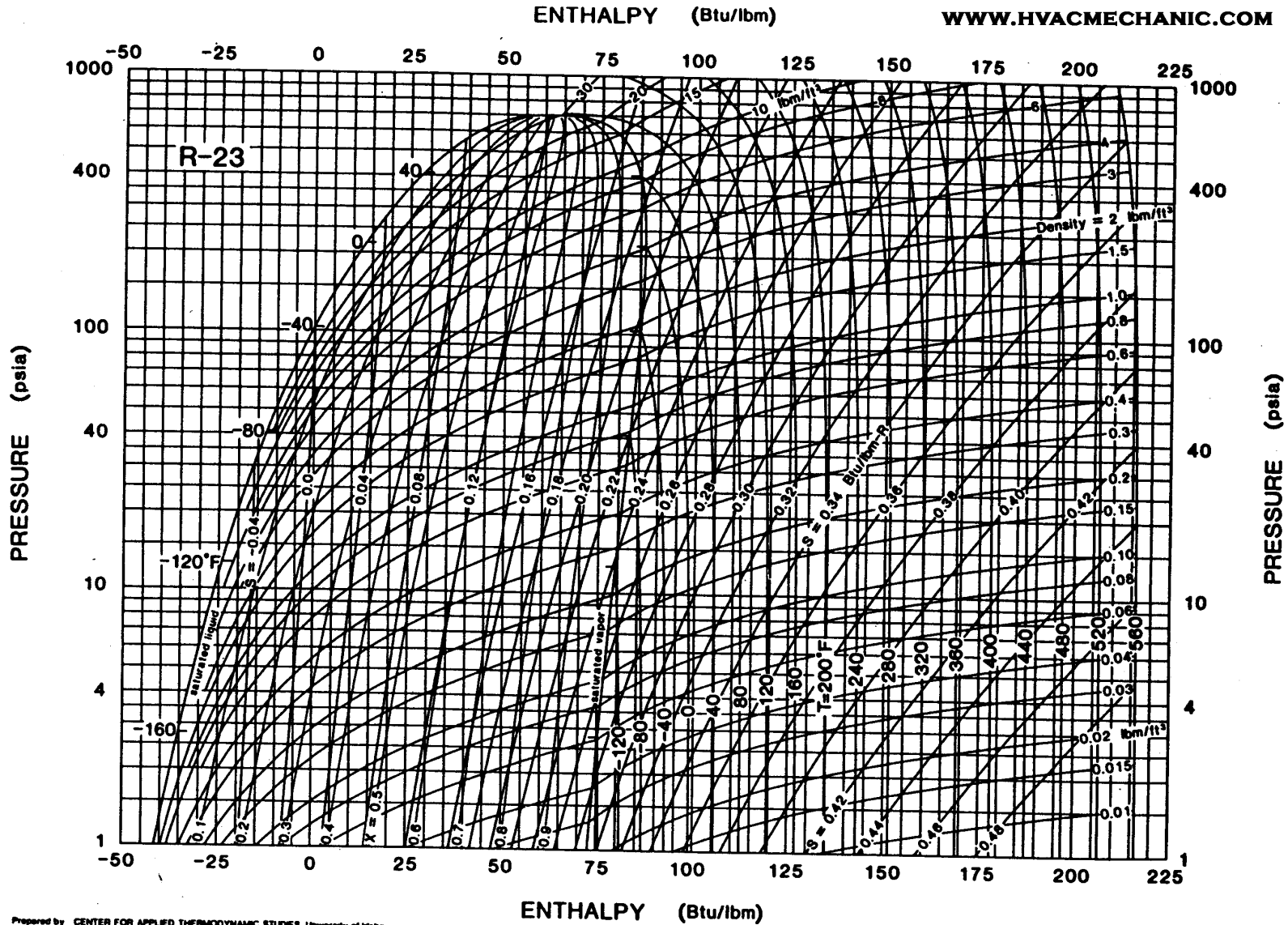
Fig. 7 Pressure-Enthalpy Diagram for Refrigerant 23
